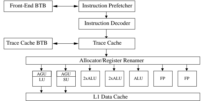
Figure 6: The Intel Netburst Microarchitecture. The execution units are LU: Load Unit; SU: Store Unit; AGU: Address Generation Unit; 2xALU: Double-speed Integer ALUs that execute two \mu\text{ops} each per cycle; ALU: Complex Integer ALU; FP: Floating Point, MMX, and SSE unit.
